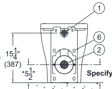
WH2135-W-2 REAR VIEW
