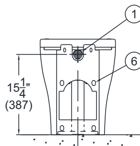
WH2135-W-3 REAR VIEW
